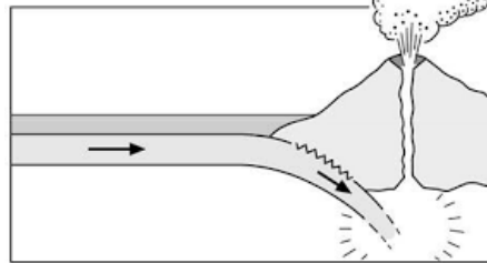
Destructive margin
