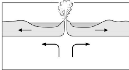
Constructive margin
